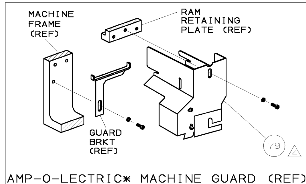
AMP-O-ELECTRIC* MACHINE GUARD (REF)
