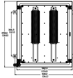
24-Pair Populated Box Part No. 7940107365
