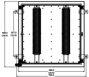
36-Pair Populated Box Part No. 7940107366
