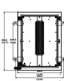
12-Pair Populated Box Part No. 7940107364
