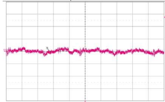
Figure 14. Input reflected-ripple current, i_s (10 mA/div.), measured through 10 \mu H at the source at full rated load current and V_{in} = 48 V . Refer to Fig. J for test setup. Time scale: 1 \mu s/div.
