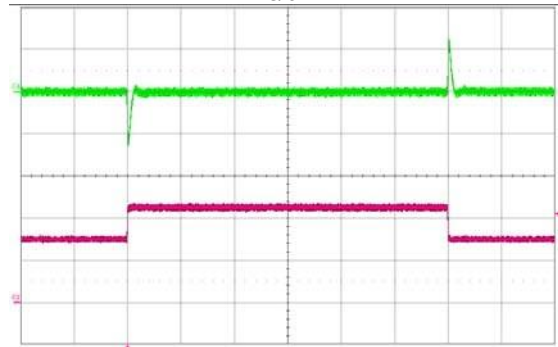
Figure 12. Output voltage response to load current step change (7.5A - 11.25A - 7.5A) at V_{in} = 48 V . Top trace: output voltage (50mV/div.) Bottom: load current (5 A/div.). Current slew rate: 1 A/ \mu s. Time scale: 200 \mu s /div. C_o = 470\mu F POS + 1 \mu F ceramic
