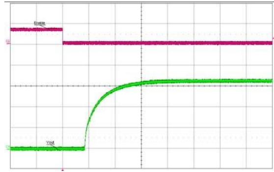
Figure 10. Turn-on waveform at full rated load current (resistive) with 10uF tant. + 1uF cer. output capacitor at V_{in} = 48V , triggered via ON/OFF pin. Top trace: ON/OFF signal (5V/div.). Bottom trace: Output voltage (1V/div.). Time scale: 2 ms/div.
