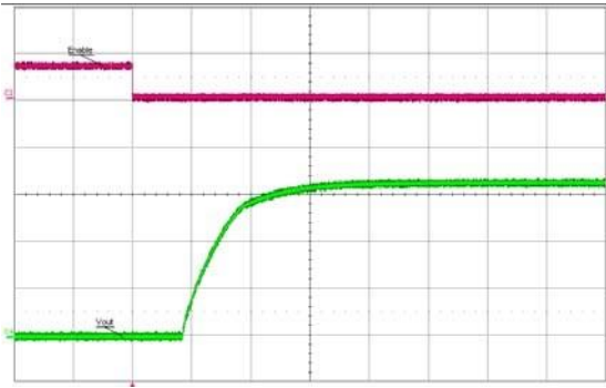
Figure 9. Turn-on waveform at full rated load current (resistive) with 7,500 uF output capacitor at V_{in}=48V , triggered via ON/OFF pin. Top trace: ON/OFF signal (5V/div.).
