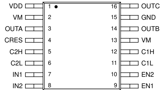
Figure 3. 17517 Pin Connections
