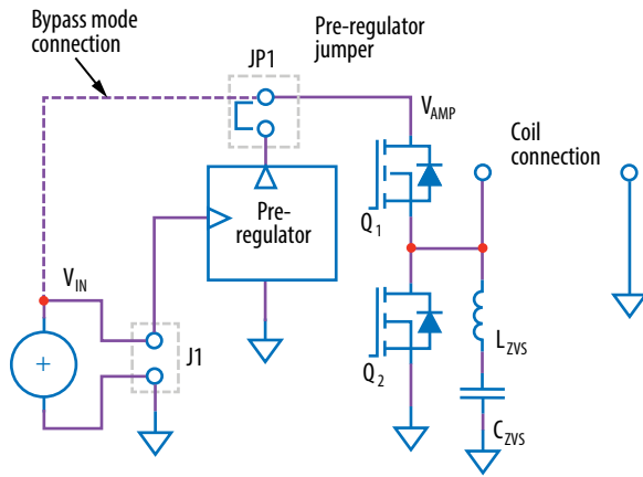
Figure 3: Diagram of EPC9510 amplifier circuit
