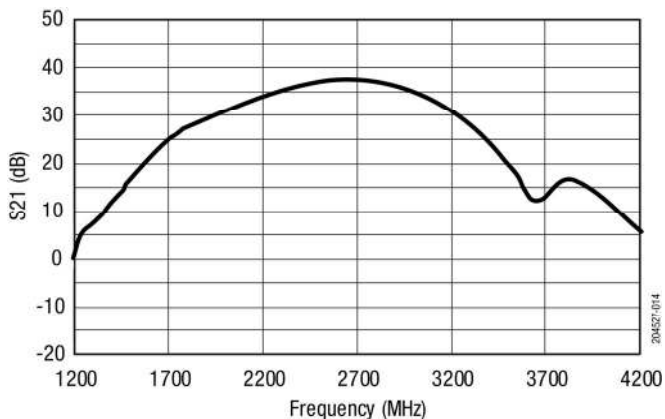
Figure 14. Wide-Band S21 vs Frequency
