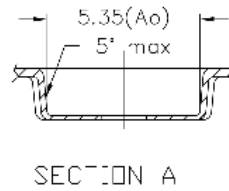
Figure 24. SKY66317-11 Tape and Reel Dimensions
