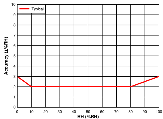
RH Accuracy (T A = 30°C)
