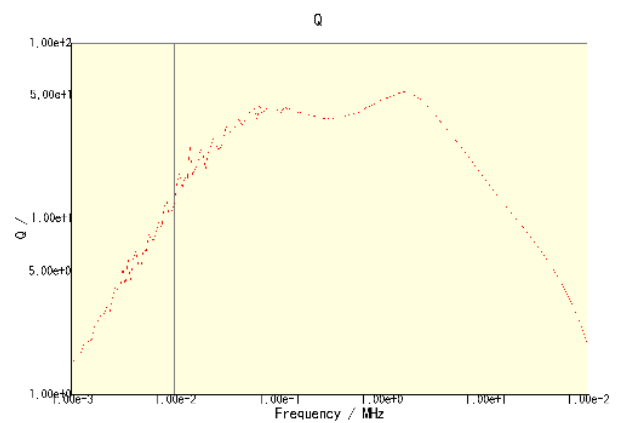
CLF6045T-1R5N-CA
