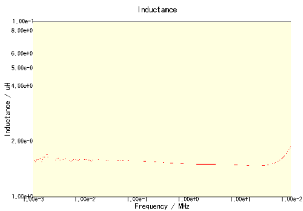
CLF6045T-1R5N-CA
