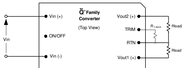
Figure 2. Configuration for increasing output voltage.
