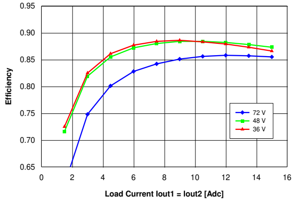
Figure 20. Efficiency vs. balanced load current (Iout1 = Iout2) and input voltage for converter mounted horizontally with air flowing from pin 3 to pin 4 at a rate of 300 LFM (1.5 m/s) and Ta = 25 °C.
