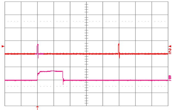
Figure 34. Load current i_{out2} into a 10\text{ m}\Omega short circuit on V_{out2} during re-start, with V_{out1} open (no load), at V_{in} = 48\text{ V} . Ch2 = i_{out2} ( 20\text{ A/div} , 20\text{ ms/div} ). ChB = i_{out2} ( 20\text{ A/div} , 1\text{ ms/div} ) is an expansion of the on-time portion of i_{out2} .
