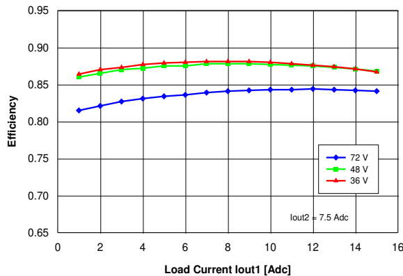
Figure 15. Efficiency vs. load current I_{out1} and input voltage for converter mounted vertically with air flowing from pin 3 to pin 1 at a rate of 300 LFM (1.5 m/s), for I_{out2} = 7.5\text{ A} and T_a = 25\text{ }^{\circ}\text{C} .
