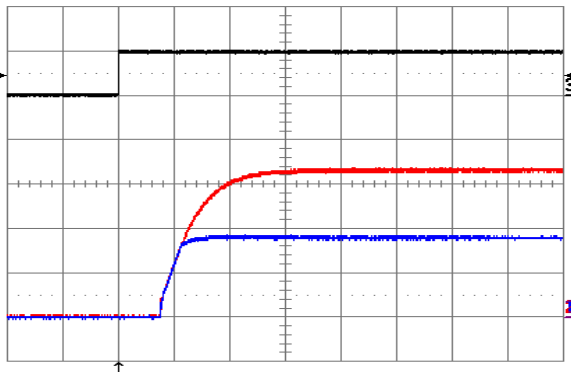
Figure 21. Turn-on transient waveforms at no load current and Vin = 48 V, triggered via ON/OFF pin. Top trace: ON/OFF signal (5 V/div.). Bottom traces: Vout1 (blue, 1 V/div.), Vout2 (red, 1 V/div.). Time scale: 1 ms/div.
