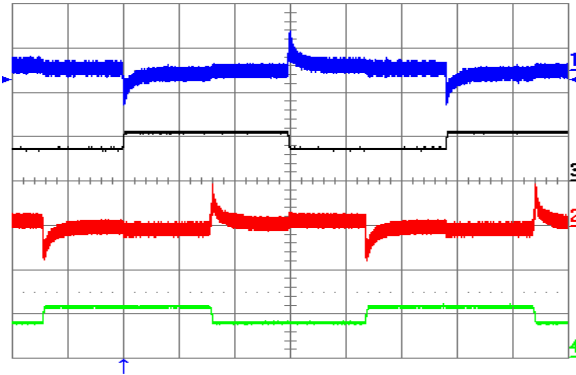
Figure 27. Output voltage response to both Iout1 and Iout2 (out of phase) load current step-change of 3.75 A (50%-75%-50%) at Vin = 48 V. Ch1 = Vout1 (50 mV/div), Ch2 = Vout2 (50 mV/div), Ch3 = Iout1 (10 A/div), Ch4 = Iout2 (10 A/div). Current slew rate: 0.1 A/μs, Co = 300 μF tantalum + 1 μF ceramic. Time scale: 1.0 ms/div.
