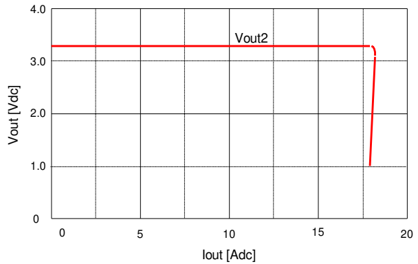
Figure 30. Output voltage Vout2 vs. load current Iout2 showing current limit point and converter shutdown point. When Vout2 is in current limit, Vout1 will follow with less than 0.6 V difference until shutdown threshold of 1 V. Input voltage has almost no effect on Vout2 current limit characteristic.
