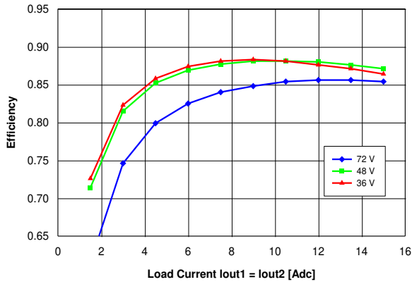
Figure 19. Efficiency vs. balanced load current (Iout1 = Iout2) and input voltage for converter mounted vertically with air flowing from pin 3 to pin 1 at a rate of 300 LFM (1.5 m/s) and Ta = 25 °C.
