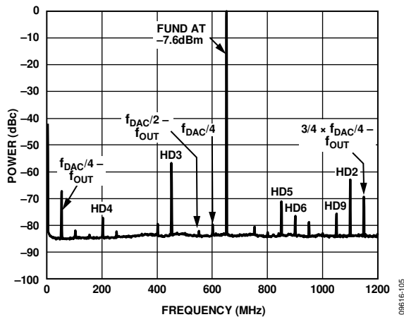
Figure 186. Spectral Plot
