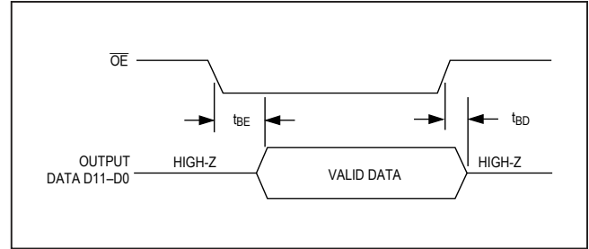
Figure 5. Output Enable Timing
