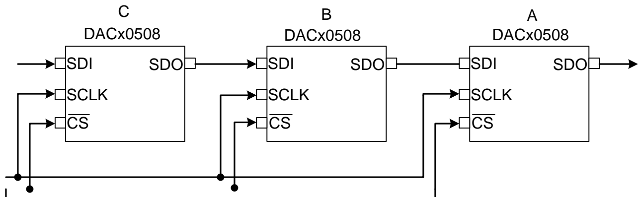
Figure 64. Daisy-Chain Layout
