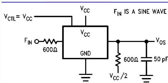
Figure 10. Switch OFF Signal Feedthrough Isolation
