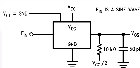
Figure 11. Sinewave Distortion
