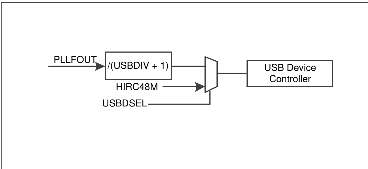
Figure 6.2-9 USB Clock Source
