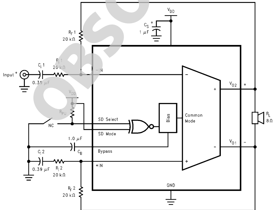
FIGURE 3. Single-Ended Input, "Shutdown-High" Configuration
