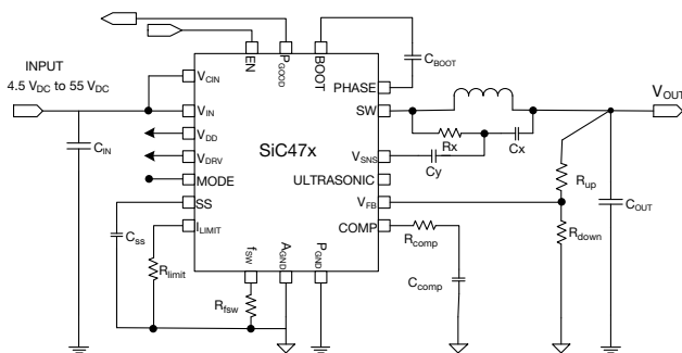
Fig. 1 - Typical Application Circuit for SiC47x
