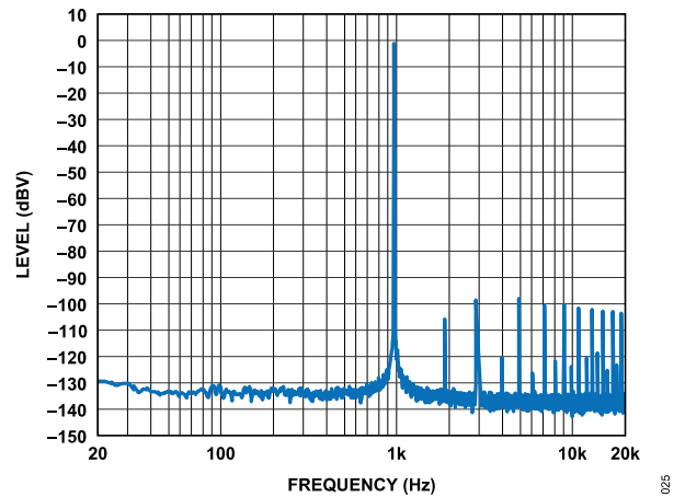
Figure 25. FFT, -1 dBFS, f_S = 48 kHz, Signal Path = SDATA1_x to the Output of the DAC Working in Headphone Mode (HPOUT), Load = 32 \Omega
