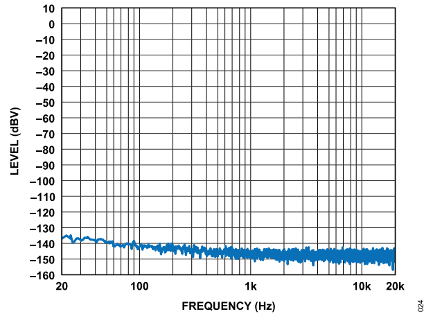
Figure 24. FFT, No Signal, f_S = 48 kHz, Signal Path = SDATA1_x to the Output of the DAC Working in Line Output Mode (LOUT), Load = 10 k \Omega
