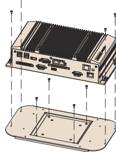
VESA mount
