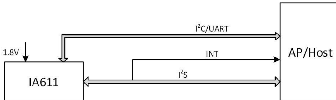
Figure 2 Application Schematic for a Host System using I2S and PC or UART
