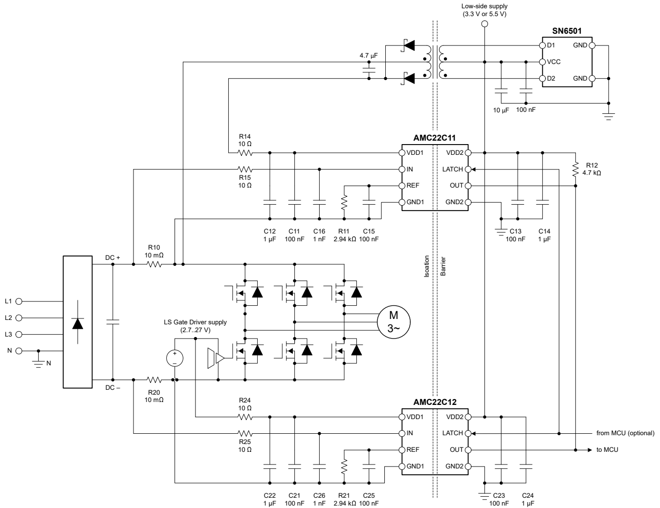
Figure 8-1. Using the AMC22C11 for DC+ Overcurrent Detection
