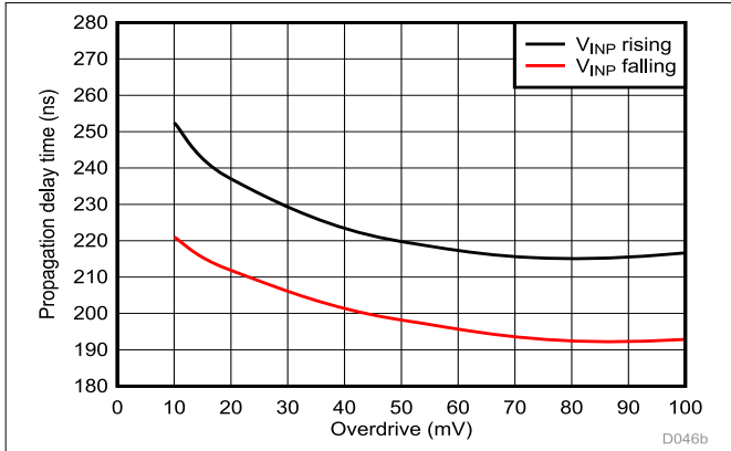
Figure 6-23. Propagation Delay vs Overdrive
