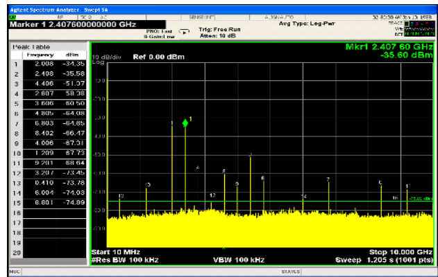
Figure 2. IF output reflection spectrum with conventional filter
