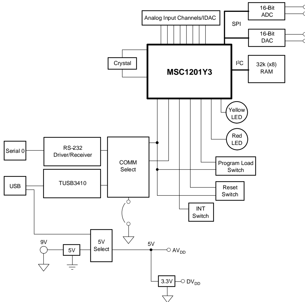
Figure 1. MSC1201/02EVM Overview
