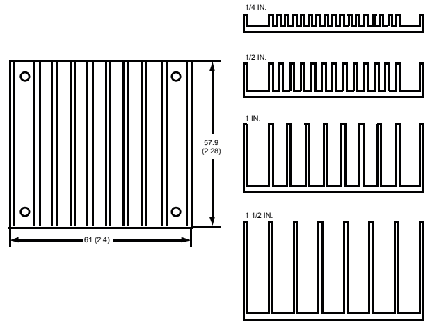
Figure 35. Transverse Heat Sink
