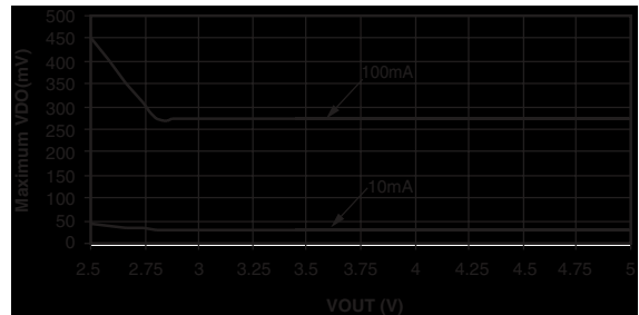
Dropout Voltage vs. Output Voltage
