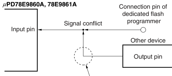
Figure 17-5. Signal Conflict (Input Pin of Serial Interface)
