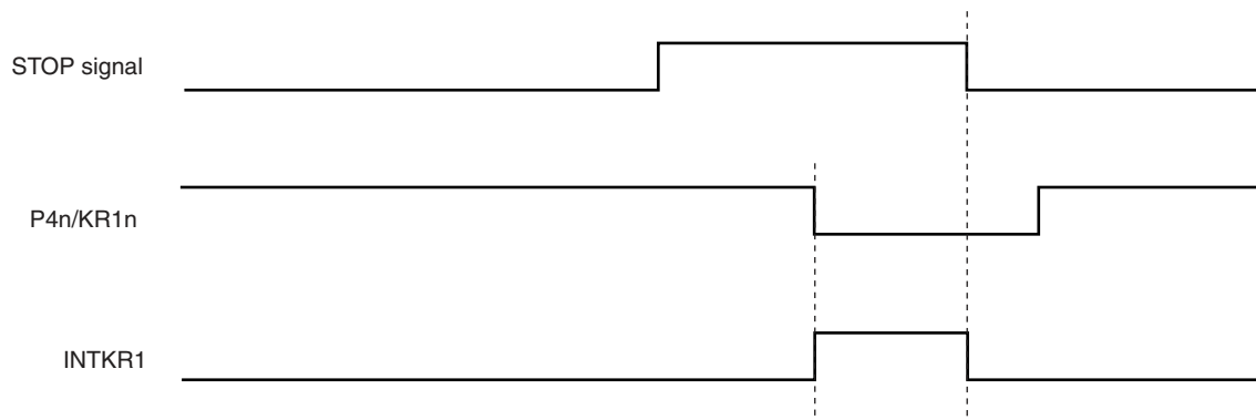
Figure 13-2. Generation Timing of Key Return Interrupt
