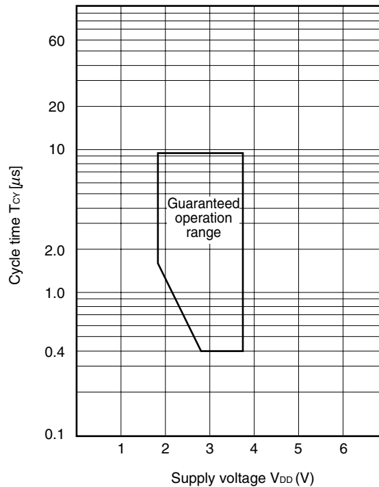
T_{CY} vs. V_{DD} (System Clock: RC Oscillation)
