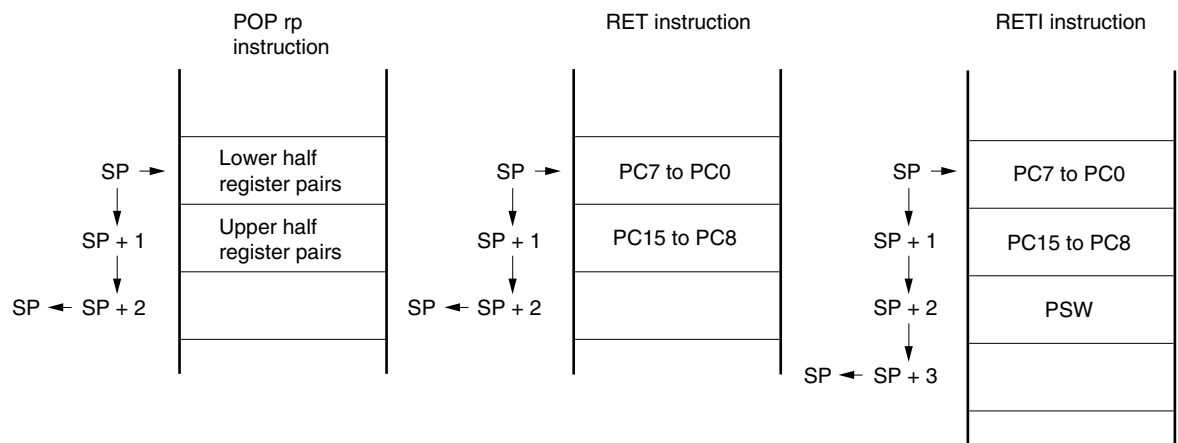
Figure 4-9. Data to Be Restored from Stack Memory
