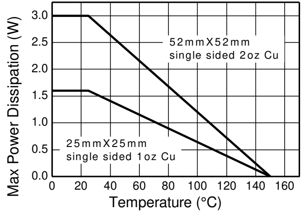
Figure 2. Derating Curve
