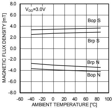
Fig.24 Bop,Brp–Ambient temperature
