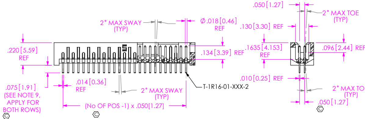
SECTION "B"-"B"
