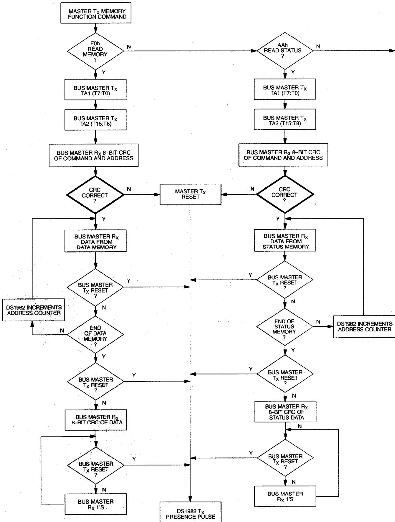
MEMORY FUNCTION FLOW CHART Figure 6
