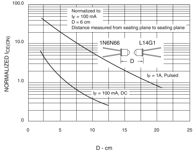
Fig. 10 I_L vs. Distance IRED/Phototransistor Pair
