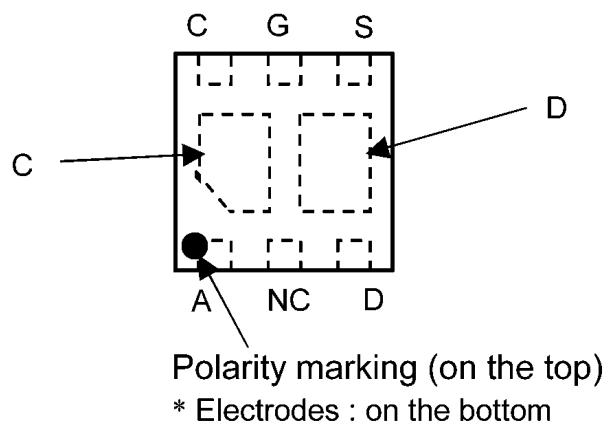
Fig. 6.2 Pin Condition(Top View)
