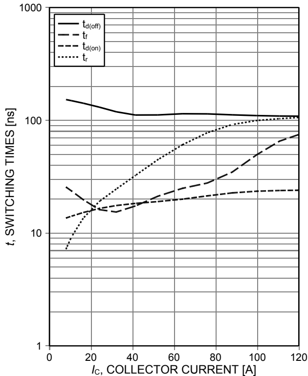
Figure 7. Typical switching times as a function of collector current (ind. load, Tj=150°C, VCE=400V, VGE=0/15V, Rg=14Ω, test circuit in Fig. E)
