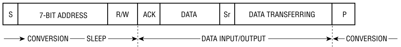
Figure 6. Conversion Sequence
