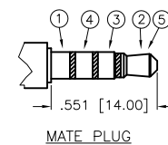
MATE PLUG
