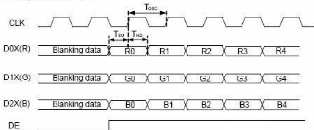
Figure4 CLK,DATA and DE wadedforms in Digital Parallel RGB
