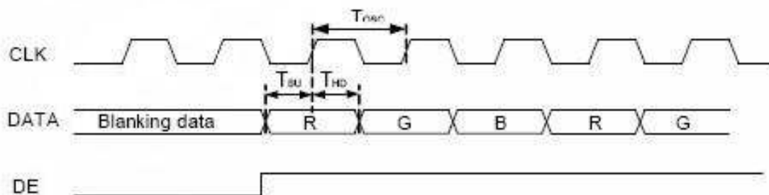
Figure3 CLK,DATA and DE waveforms in Digital Serial RGB
