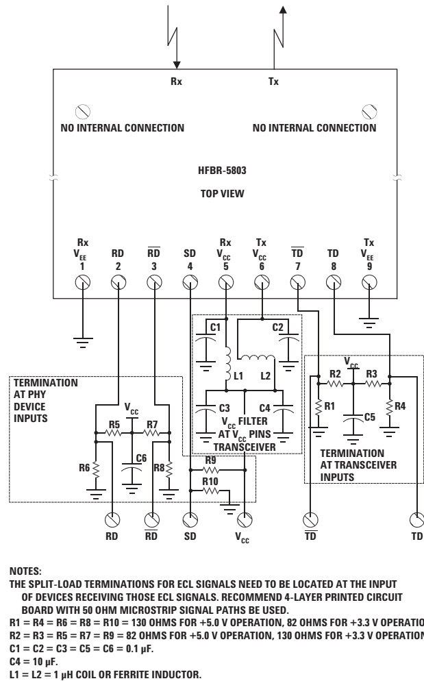
Figure 7. Recommended Decoupling and Termination Circuits
