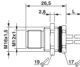
Dimensioned drawing
