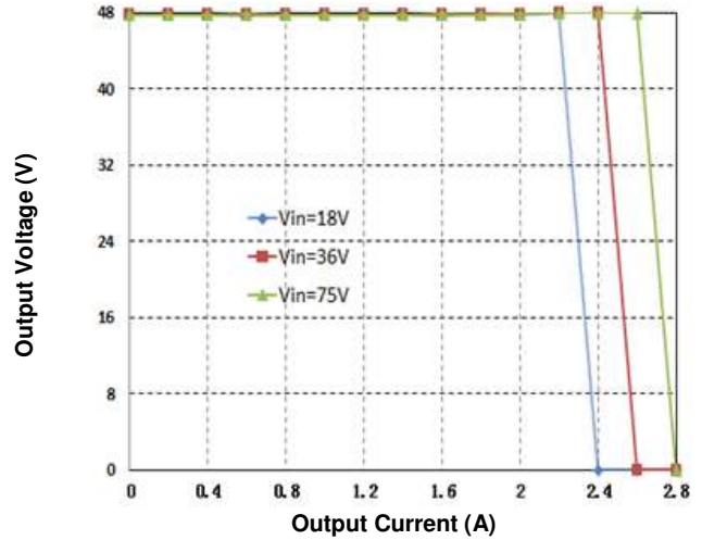
Figure 2. Output Characteristics (25°C)
