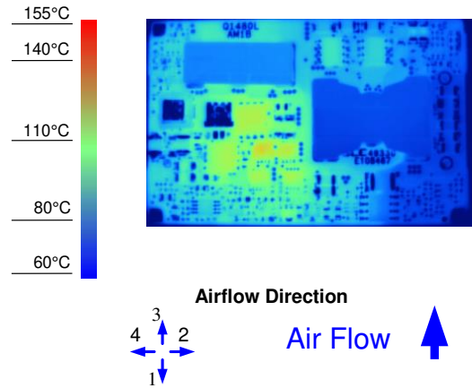
Figure 8. Thermal Image for Airflow Direction 3 (2A output, 55°C ambient, 200 LFM, typical Vin, open frame, unit soldered onto a fixture board)
