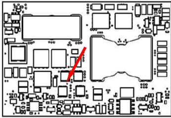
Figure 14. Temperature Monitoring Locations
