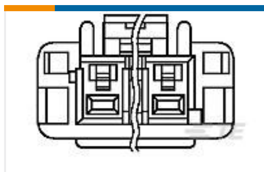
TE Part #2-1376389-3 5MM POWER KEY 3P PLUG HSG BLUE
