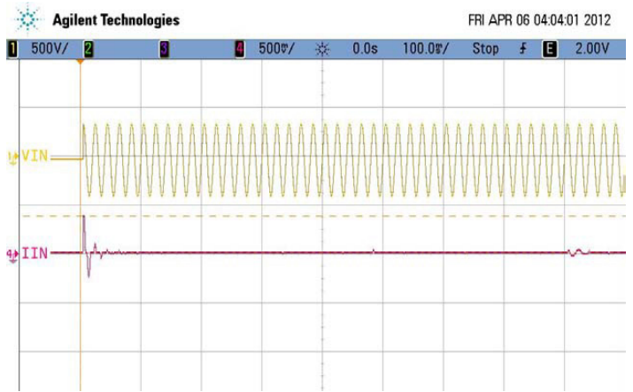
Inrush Current
