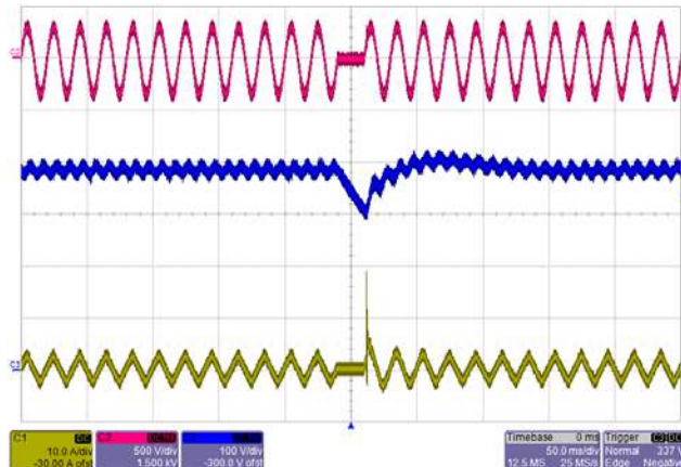
Figure 40 – Line Dropout 230 VAC, 50 Hz Top: Input Voltage, 500 V / div. Middle: Output Voltage, 100 V / div. Bottom: Input Current, 10 A, 50 ms / div.
