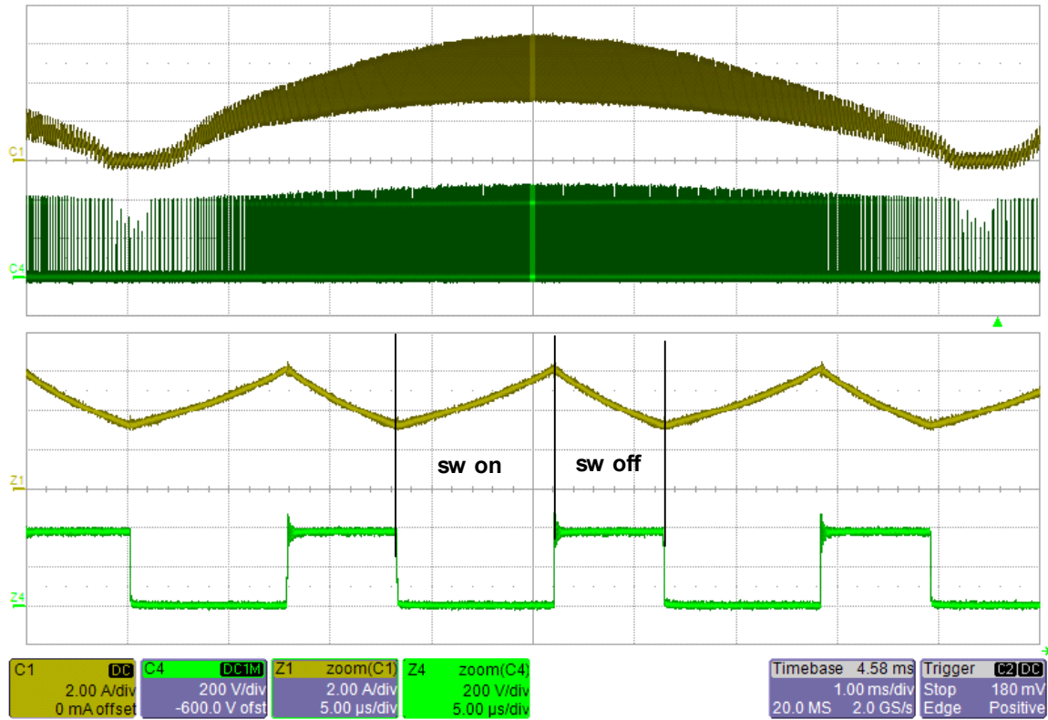
Figure 80 – 115 VAC, 100% Load. Top: Inductor Current, 2 A / div. Bottom: Drain Voltage, 200 V / div. Zoom Top: Inductor Current, 2 A, 5 μs / div. Zoom Bottom: Drain Voltage, 200 V / div., 5 μs / div.
