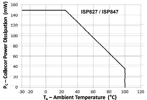
Fig 4 Collector Power Dissipation vs Ambient Temperature (2)
