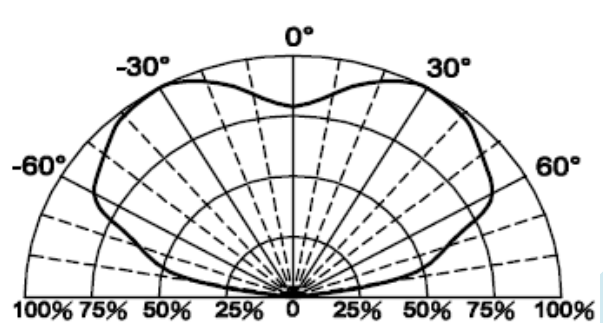
Fig.6 Directive Radiation
