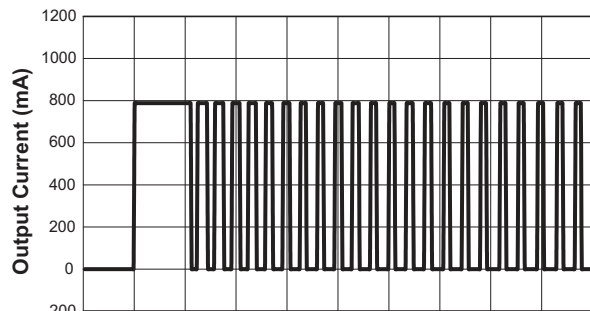
Over-Current Protection
