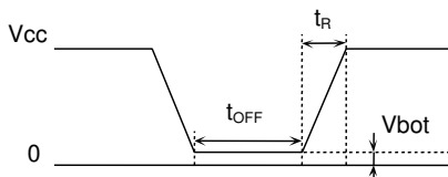
Figure 60. Rise waveform
