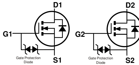
Device Symbol
