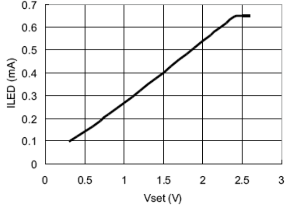
12. I LED VS V SET (V IN =16V, 3 LEDs, 47µH, R S =0.15Ω)
