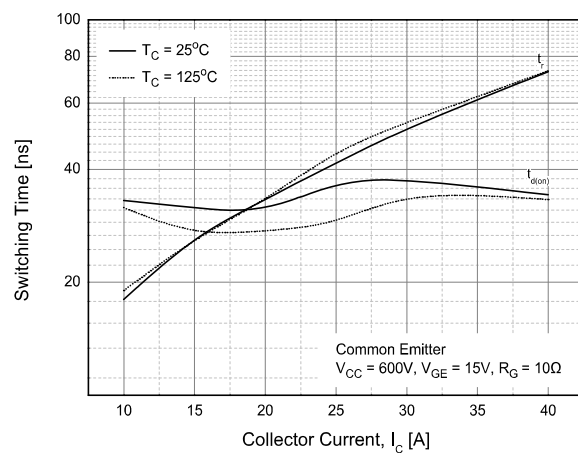
Fig. 10 Turn on time vs. collector current
