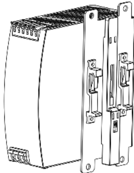
Side mounting with DIN-rail brackets
