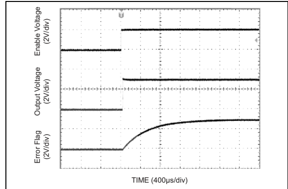
FIGURE 2-22: Error Flag Start-Up (see Figure 1-1).
