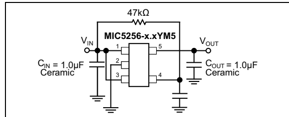
FIGURE 4-1: Low-Noise Fixed Voltage Application.
