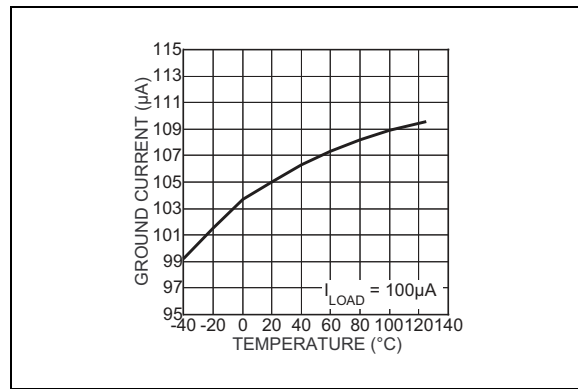
FIGURE 2-5: Ground Pin Current.
