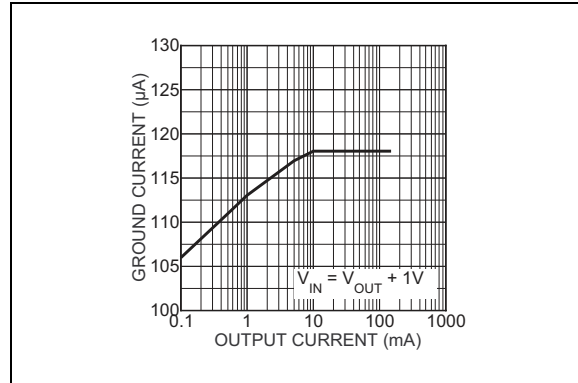
FIGURE 2-4: Ground Pin Current.
